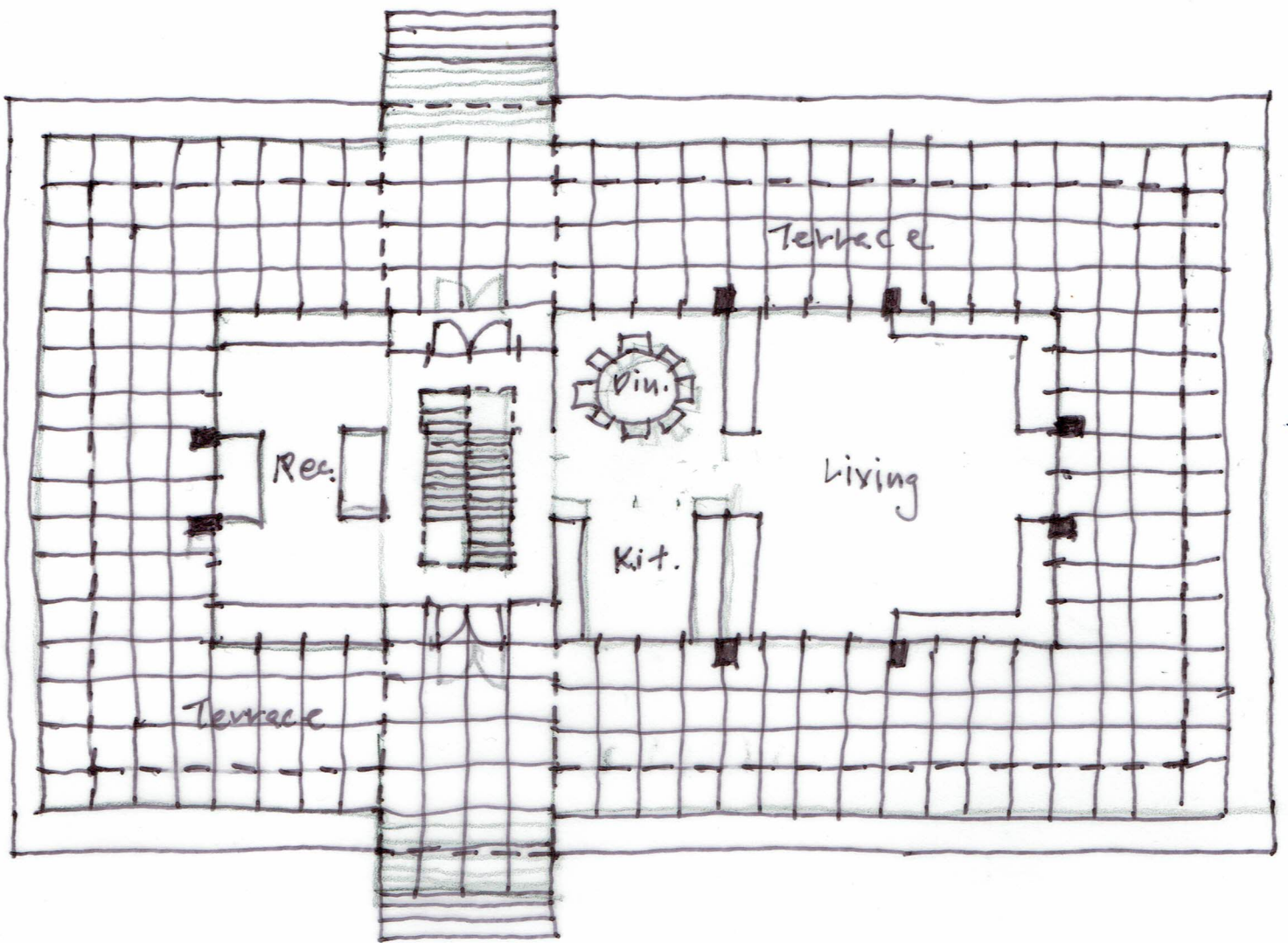
1st. Floor Plan: Single Family 3 rd Bed. House Scale: \frac{1}{4}'' = 3'-0''
