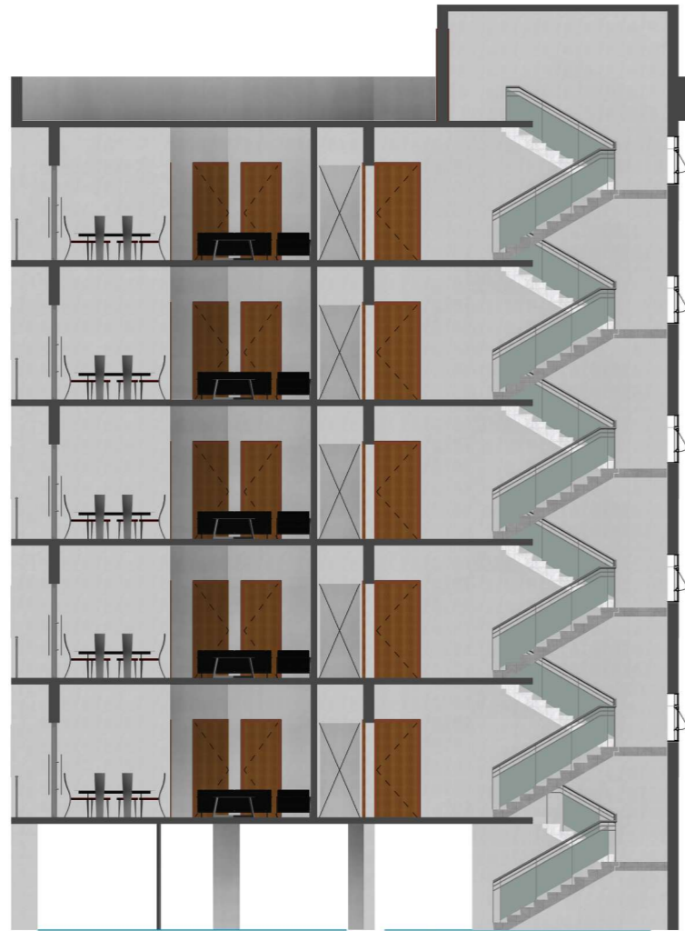
BLOCK 1 - SECTION 1 SCALE 1 : 100
